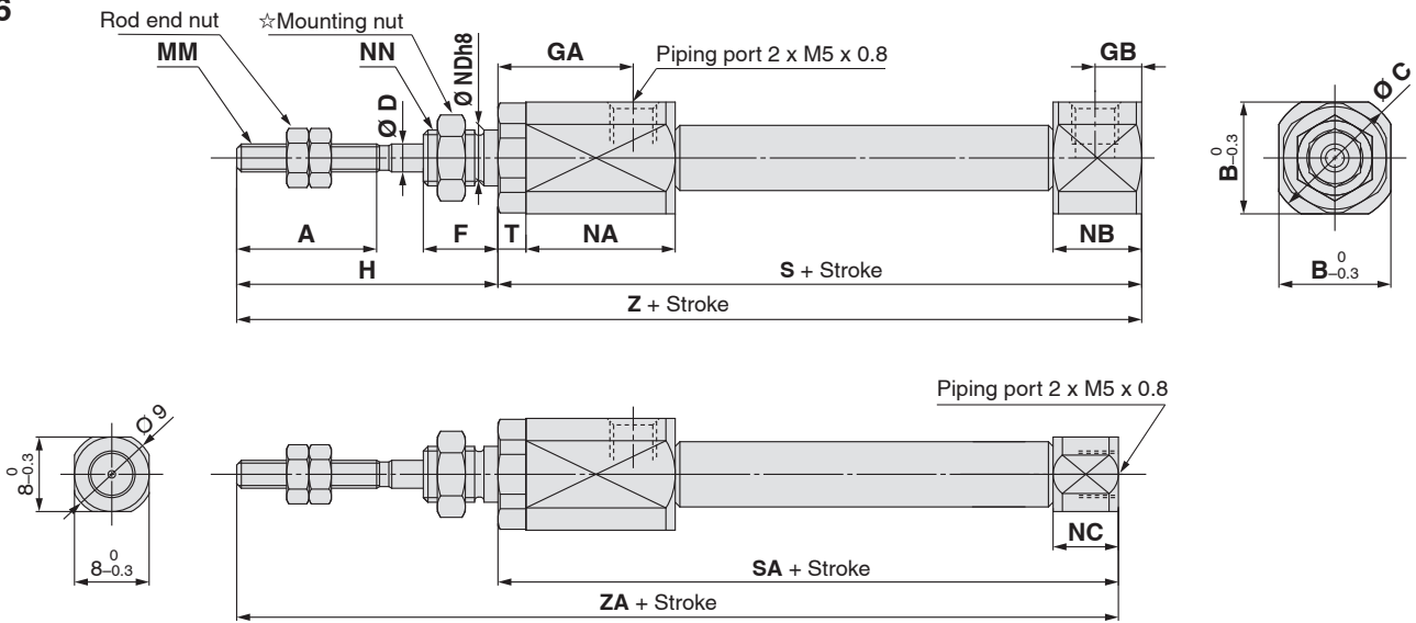
Head cover port location Axial location (R)
